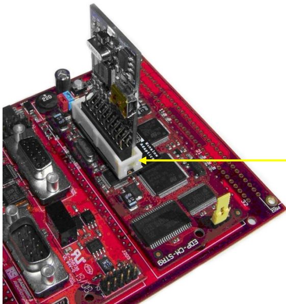
Correct orientation of the dongle on the CM module
